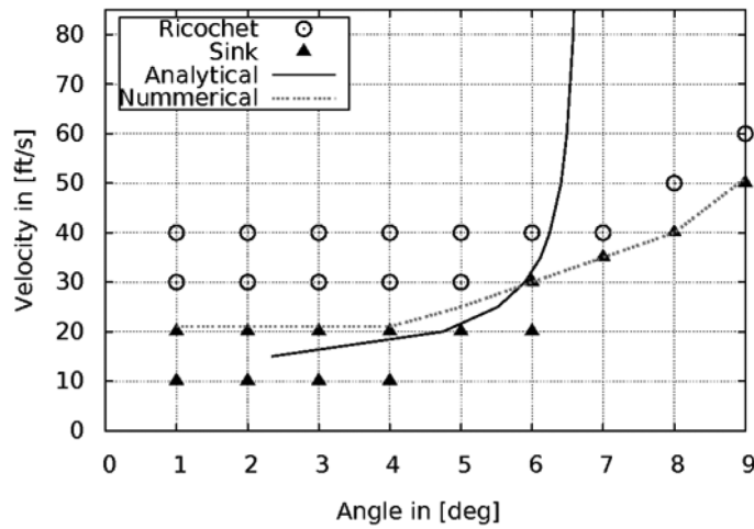
Figure 7: SPH ricochet perdition of cylinder; triangles for sink and circles for ricochet; dotted line shows ricochet behaviour of ALE model
