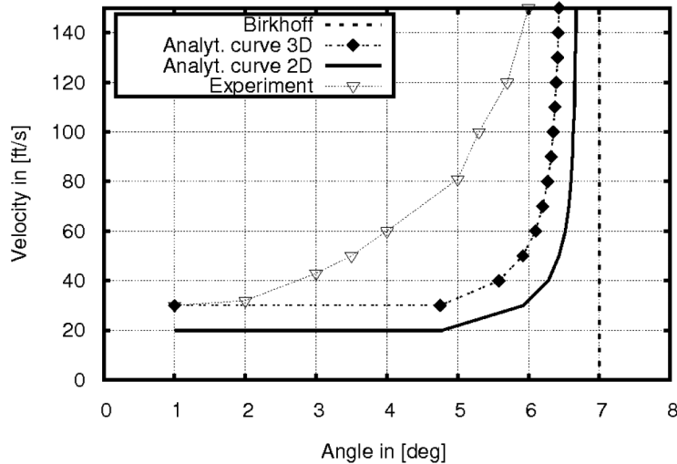
Figure 2: Analytical models plotted with experimental data for 2D and 3D impact case on water
