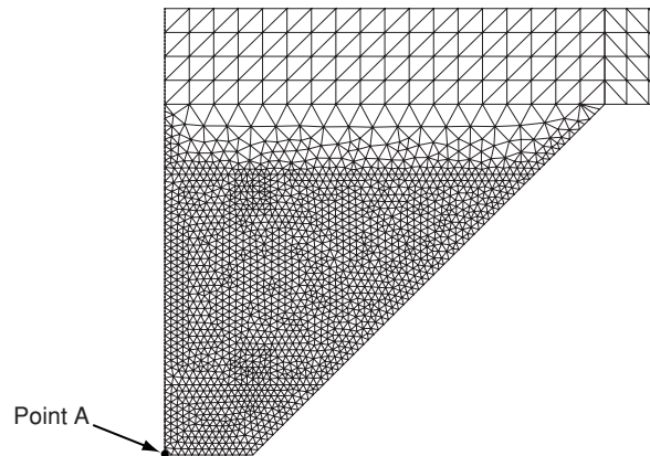
Figure 3 Meshing details in the conical part of the pin.
