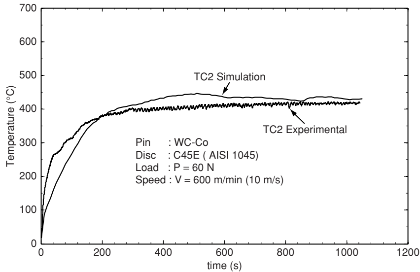
Figure 7 Comparison between the experimental and numerical (approach 1) temperature evolutions during a tribological test performed at a 600 m/min sliding speed and under a 60 N normal loading: case of the TC2 thermocouple.
