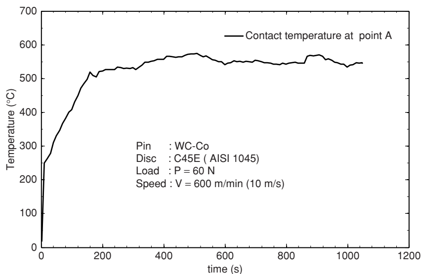
Figure 8 Evolution of the estimated contact temperature at point A (approach 1) in the case of tribological test performed at a 600 m/min sliding speed and under a 60 N normal loading.
