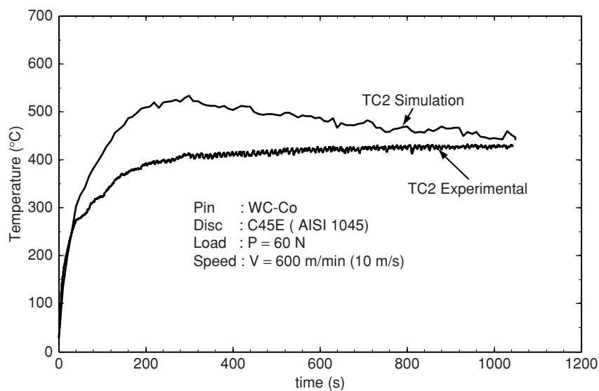
Figure 10 Comparison between the experimental and numerical (approach 2) temperature evolutions during a tribological test performed at a 600 m/min sliding speed and under a 60 N normal loading: case of the TC2 thermocouple.
