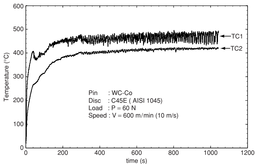
Figure 5 Temperature (measured by TC1 and TC2 thermocouples) versus sliding time during a tribological test performed at a 600 m/min sliding speed and under a 60 N normal loading.
