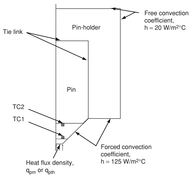
Figure 2 Axisymmetric configuration of the pin, of the pin-holder and boundary conditions (for a V = 600 m/min sliding speed).
