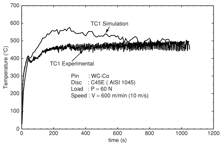
Figure 9 Comparison between the experimental and numerical (approach 2) temperature evolutions during a tribological test performed at a 600 m/min sliding speed and under a 60 N normal loading: case of the TC1 thermocouple.
