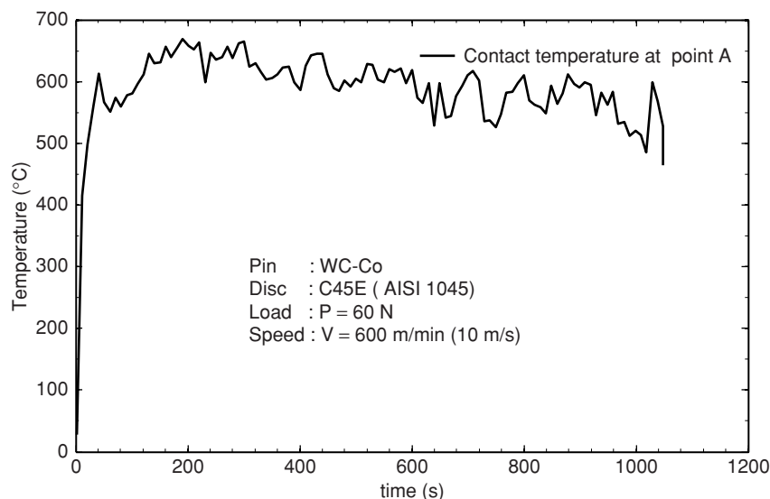
Figure 11 Evolutions of the estimated contact temperature at point A (approach 1 and approach 2) in the case of tribological test performed at a 600 m/min sliding speed and under a 60 N normal loading.
