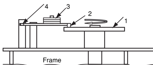
Figure 1 Tribometer description.
