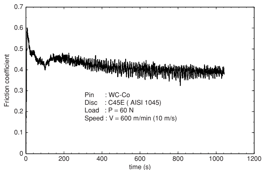
Figure 4 Friction coefficient versus sliding time during a tribological test performed at a 600 m/min sliding speed and under a 60 N normal loading.
