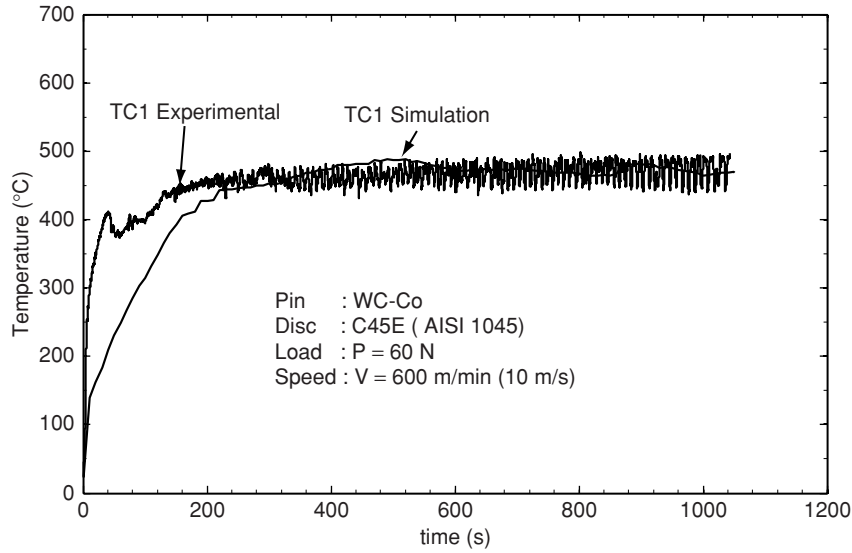
Figure 6 Comparison between the experimental and numerical (approach 1) temperature evolutions during a tribological test performed at a 600 m/min sliding speed and under a 60 N normal loading: case of the TC1 thermocouple.
