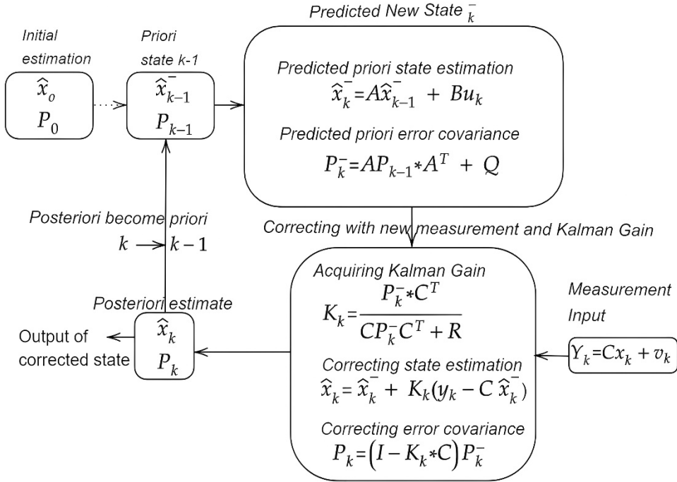
Fig.7. Recursive Kalman Filter predictor-corrector algorithm.
