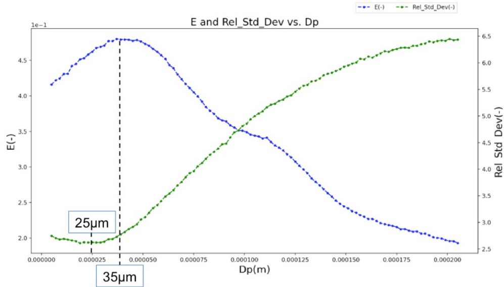
Figure 8. Combined results of 100 individual simulation runs where Mean particle diameters were varied in 100 steps between 5\mu\text{m} and 205\mu\text{m} . Coating efficiency ( E , blue) and Relative Standard batch-based coating deviation ( \text{Rel\_Std\_Dev}(-) , green) against Mean particle diameters ( D_p ). See also [27].
