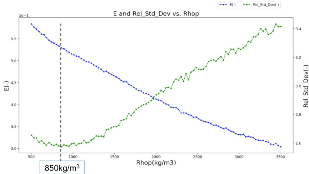
Figure 13. Combined results of 100 individual simulation runs where Particle density was varied in 100 steps between 500 \text{ kg/m}^3 and 3500 \text{ kg/m}^3 . Coating efficiency ( E , blue) and relative Standard batch-based coating deviation ( \text{Rel\_Std\_Dev} , green) against Particle density ( \text{Rhop} ).
