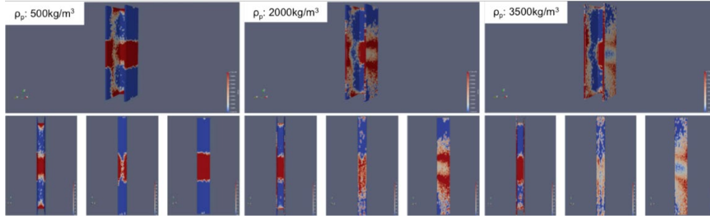
Figure 12. Simulated coating patterns (visualization of Volume fraction fields) for varying Particle densities: 500 \text{ kg/m}^3 (left), 2000 \text{ kg/m}^3 (centre) and 3500 \text{ kg/m}^3 (right). Top row shows front-side view of U-profile substrate and bottom row shows front- (left), back- (centre) and side- (right) view of U-profile per powder Particle density setting.
