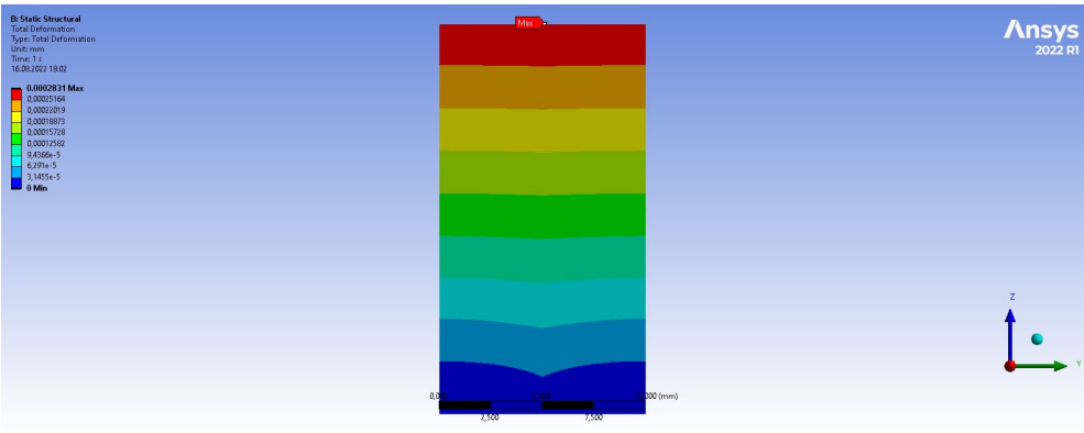
Figure 16: Max. Deformation (mm) and Von-Mises stress (MPa) of Configuration 4 (volume: 1348.4 mm 3 ), infill ratio of 64%
