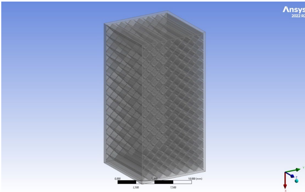
Figure 8: CAD Model and FEA Mesh of Configuration 2 (volume: 538.02 mm 3 ), infill ratio of 19%
