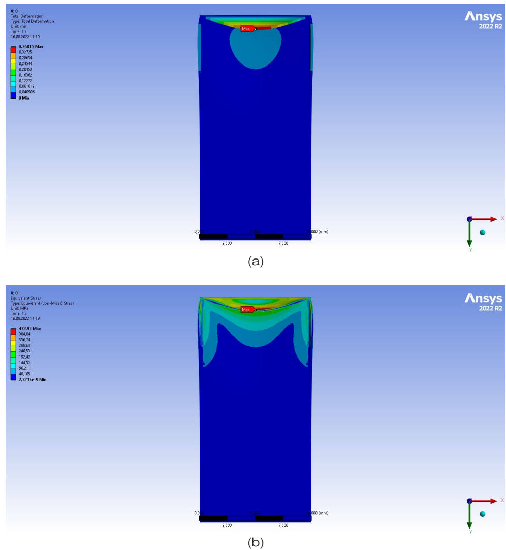
Figure 12: Max. Deformation (mm) and Von-Mises stress (MPa) of Configuration 0 (volume: 192.824 mm 3 ), infill ratio of 0%
