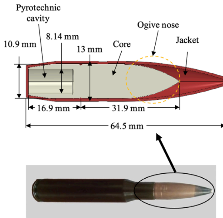
Figure 2: Cross-sectional view of the 12.7 mm AP tracer projectile revealing the core and the pyrotechnic cavity.
