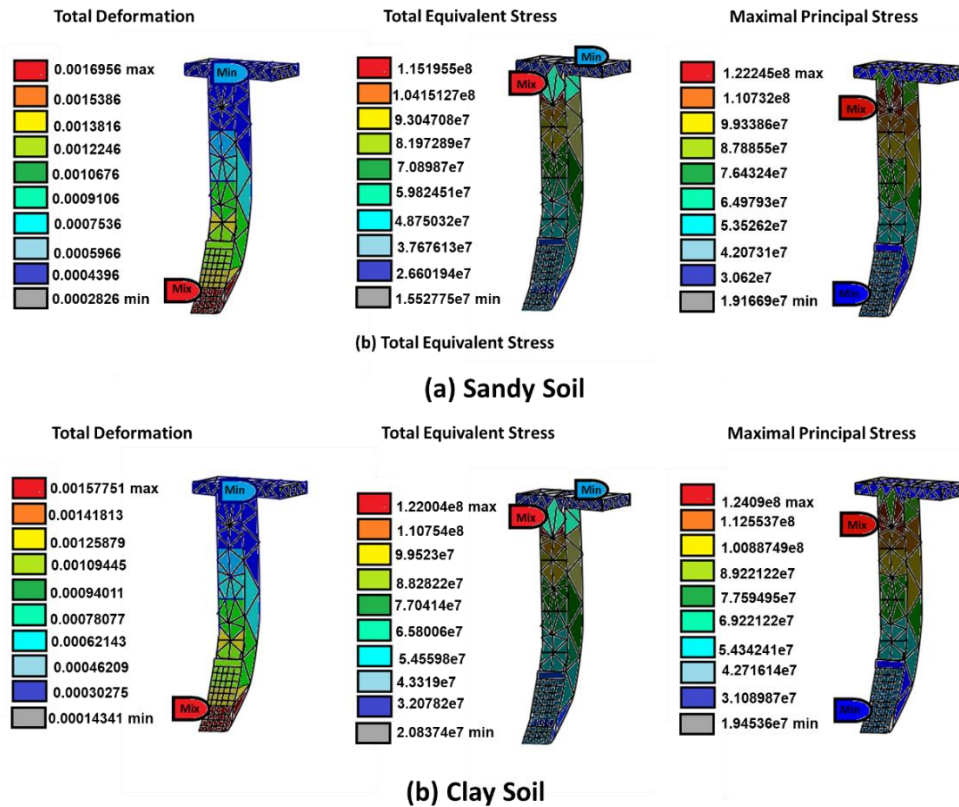
Figure 7: Deformation and Principal Stresses
