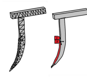
Figure 5: Boundary condition
