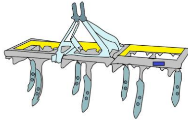
Figure 2: Geometric CAD modal
