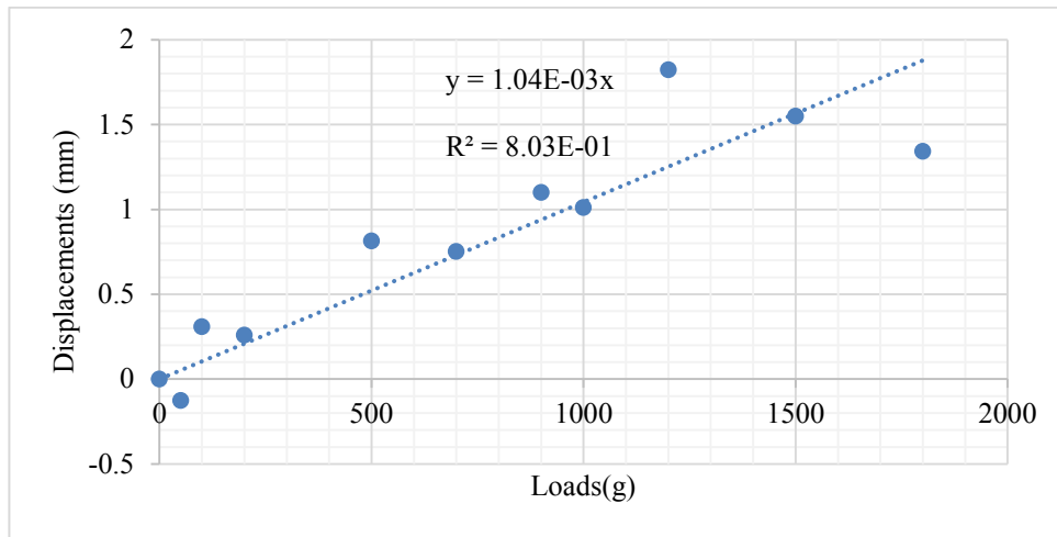
Figure 10: Displacement with variation in load for 3 mm thick ice sample
