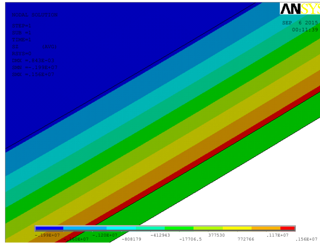
Figure 18: Zoomed-in view of longitudinal stress in the sample with 5 mm ice thickness loaded under 3500g.
